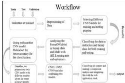
Fig. 2. Workflow Representation
